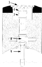
B. Overfill Prevention with OPW 61SOR
