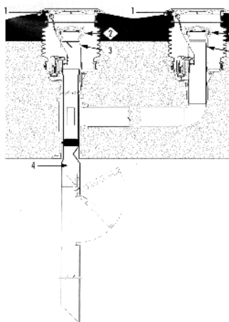
B. Overfill Prevention with OPW 61SOR
