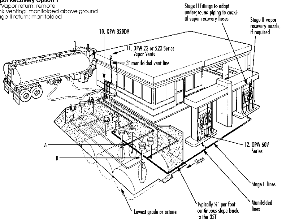
A. Overfill Prevention with the OPW 53VMI.
